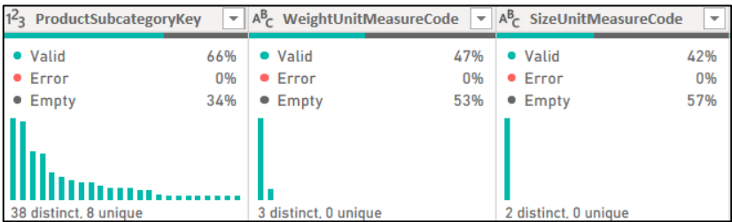
Figure 3: Null cells that will need fixing
